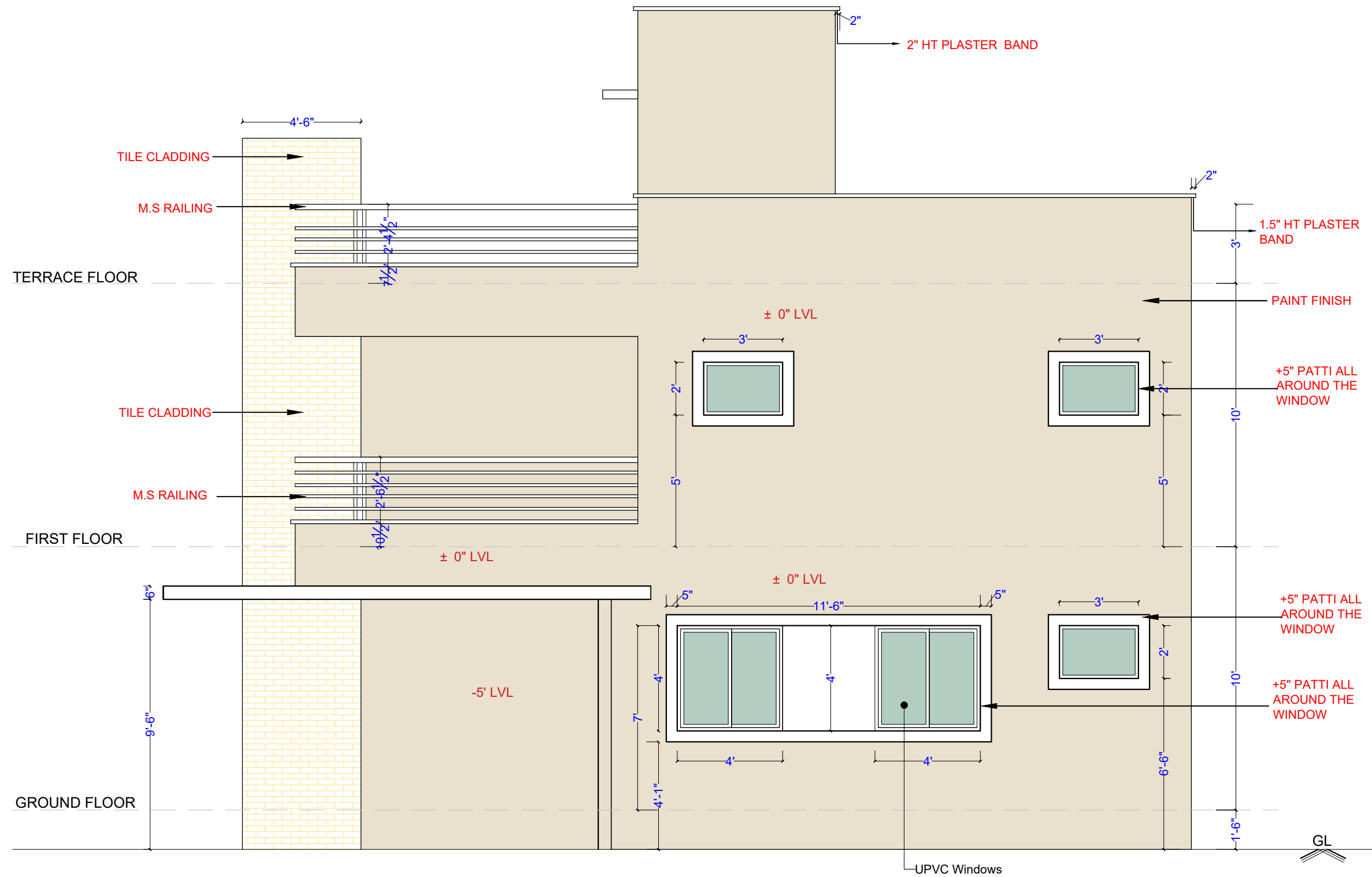
NORTH ELEVATION
