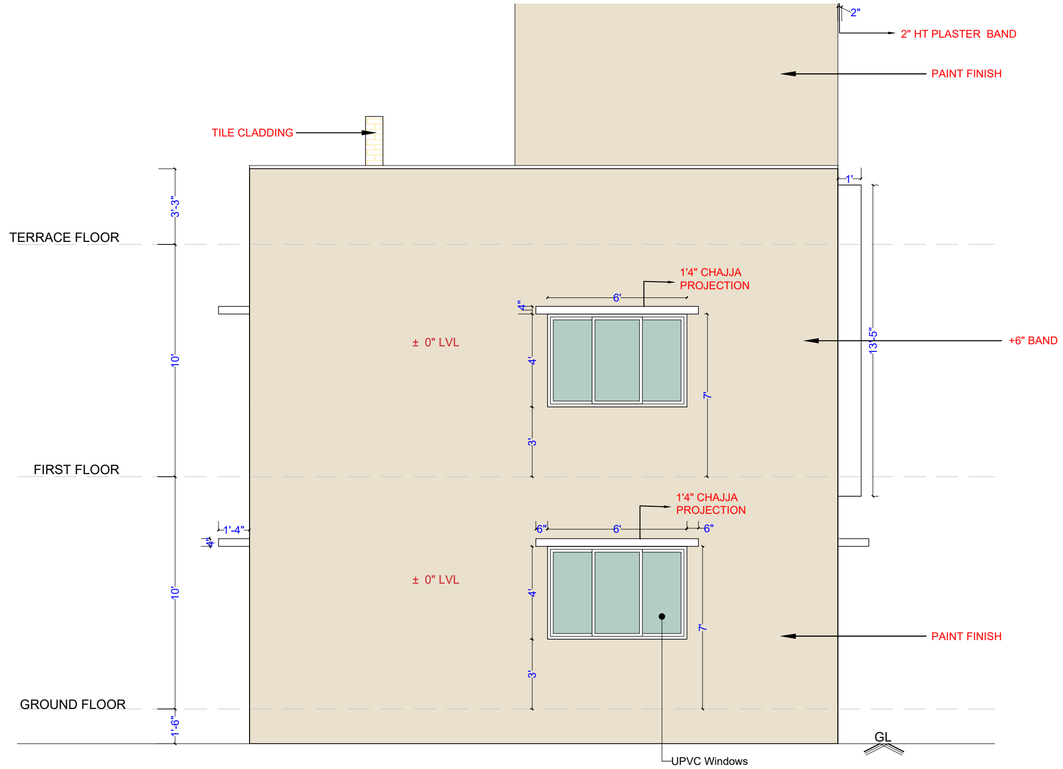
WEST ELEVATION
