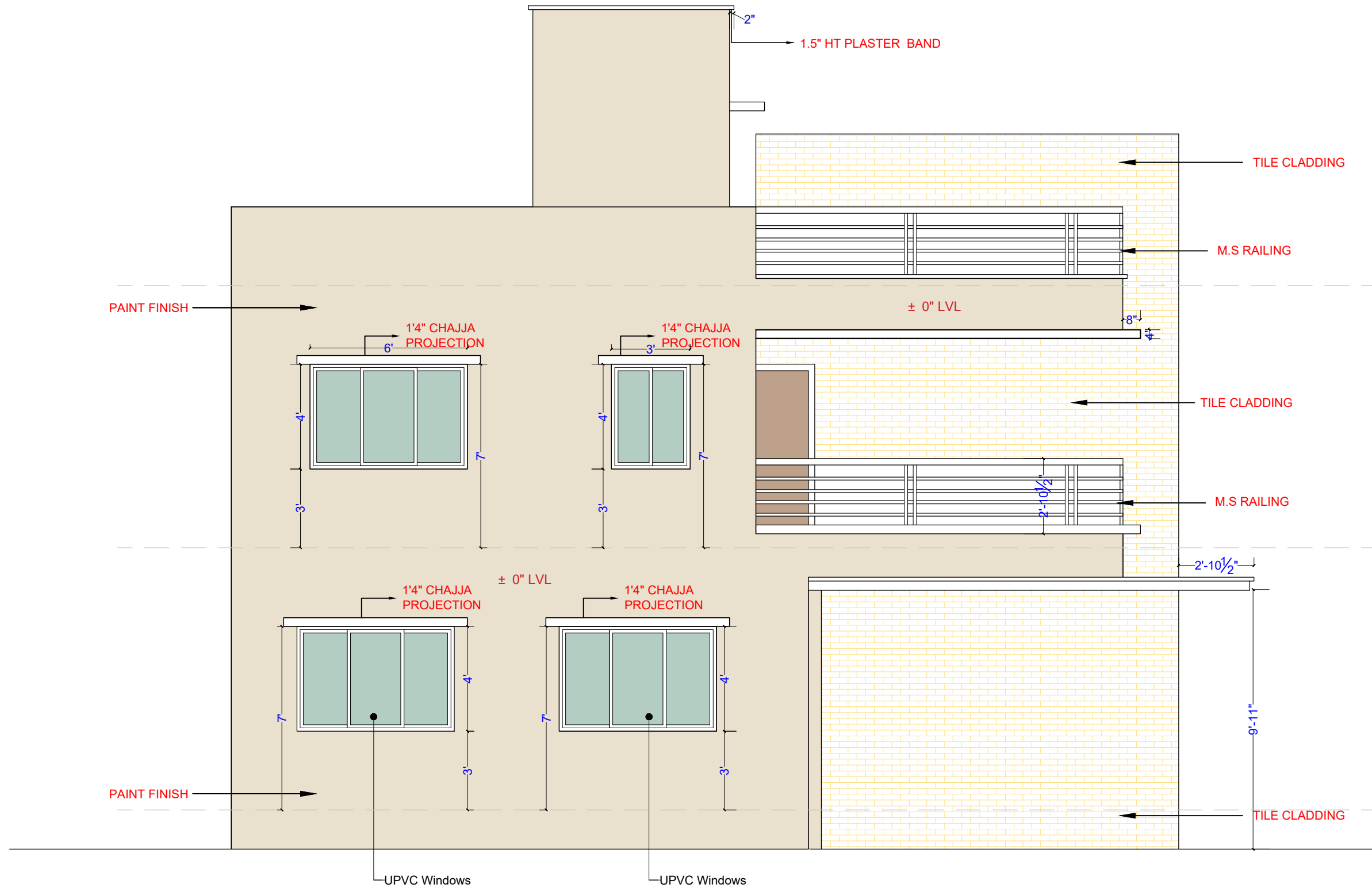
NORTH ELEVATION
