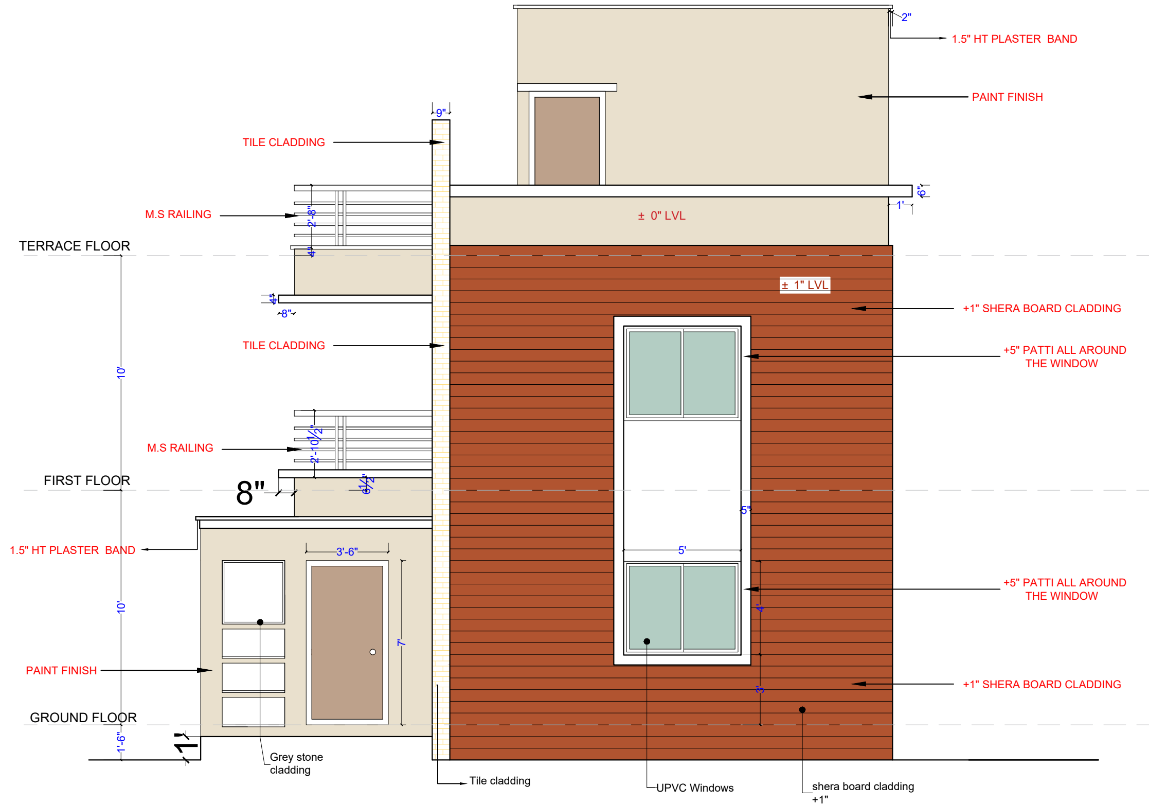
WEST ELEVATION
