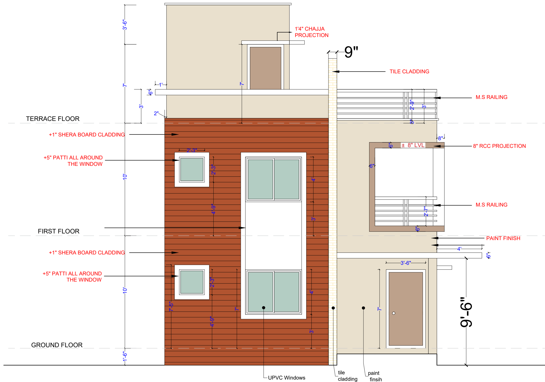
EAST ELEVATION
