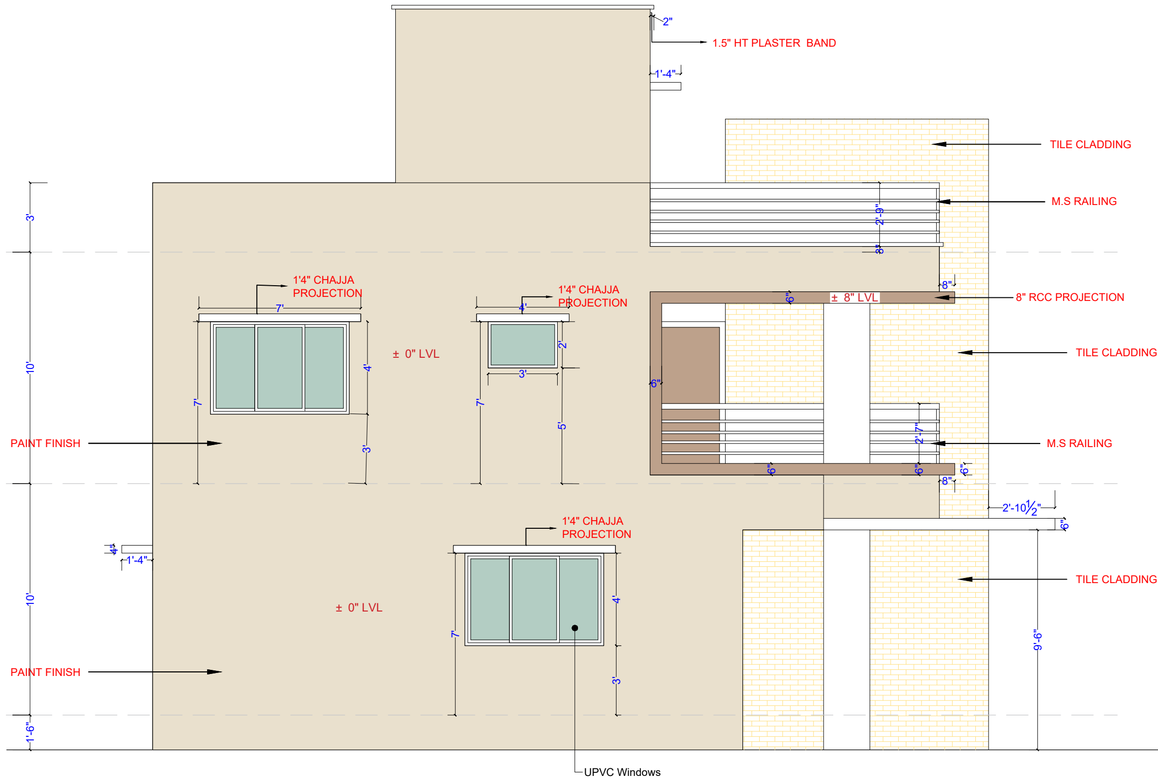
NORTH ELEVATION
