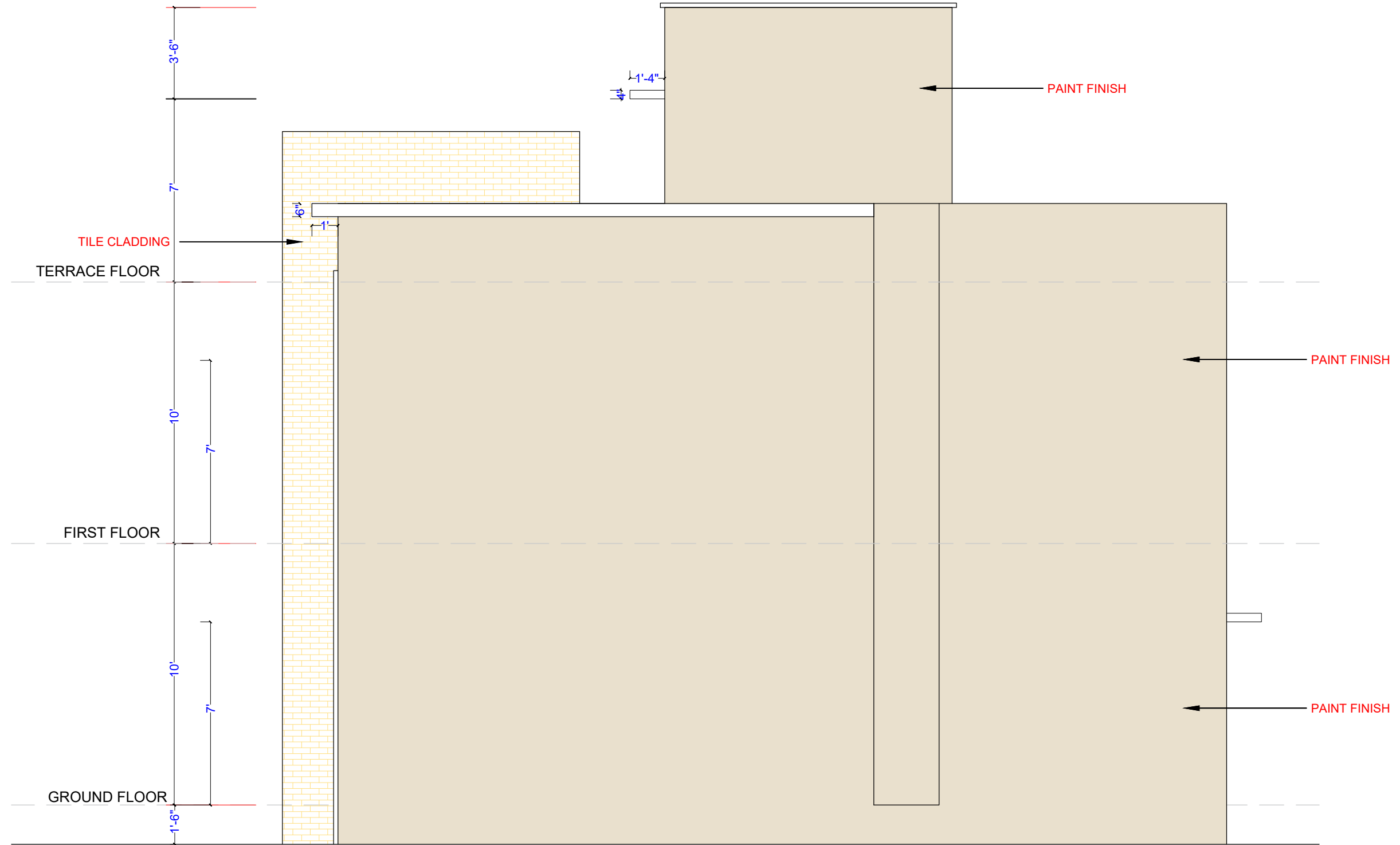
SOUTH ELEVATION
