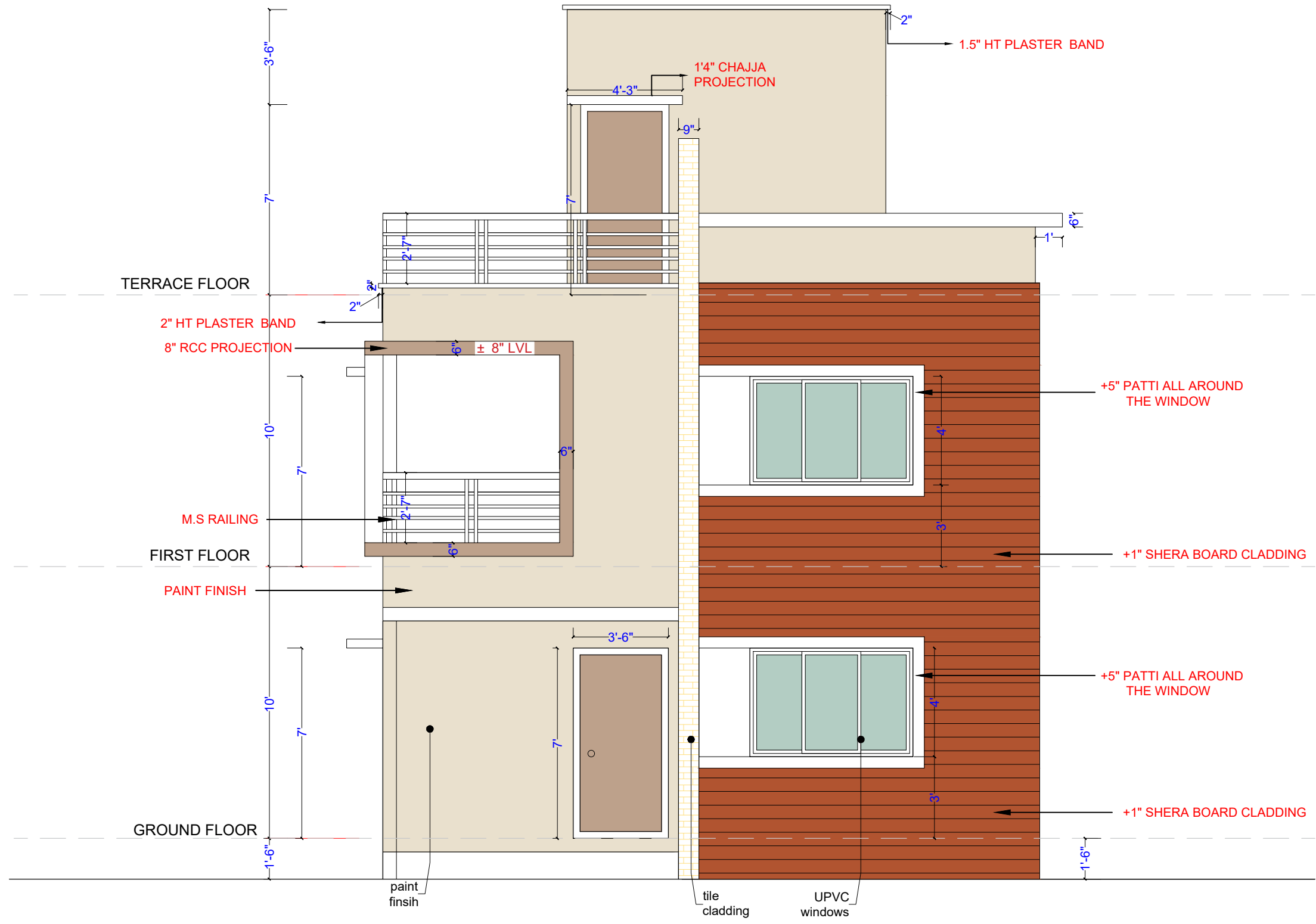
WEST ELEVATION
