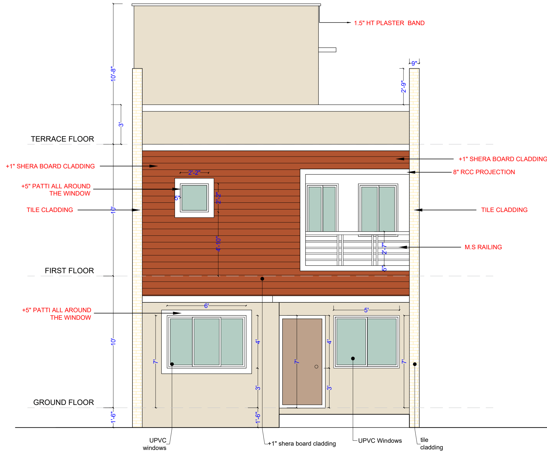
EAST ELEVATION
