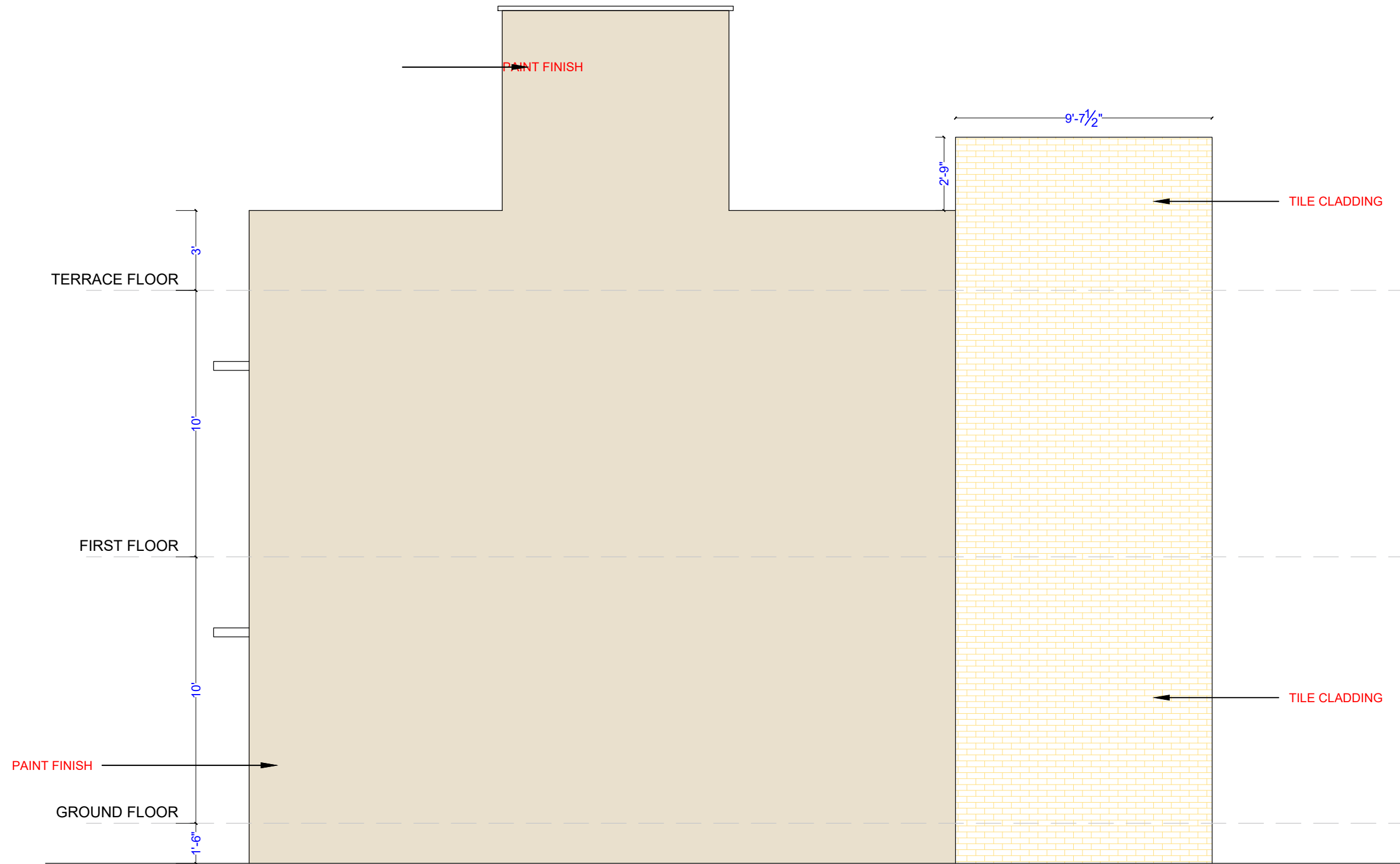
SOUTH ELEVATION
