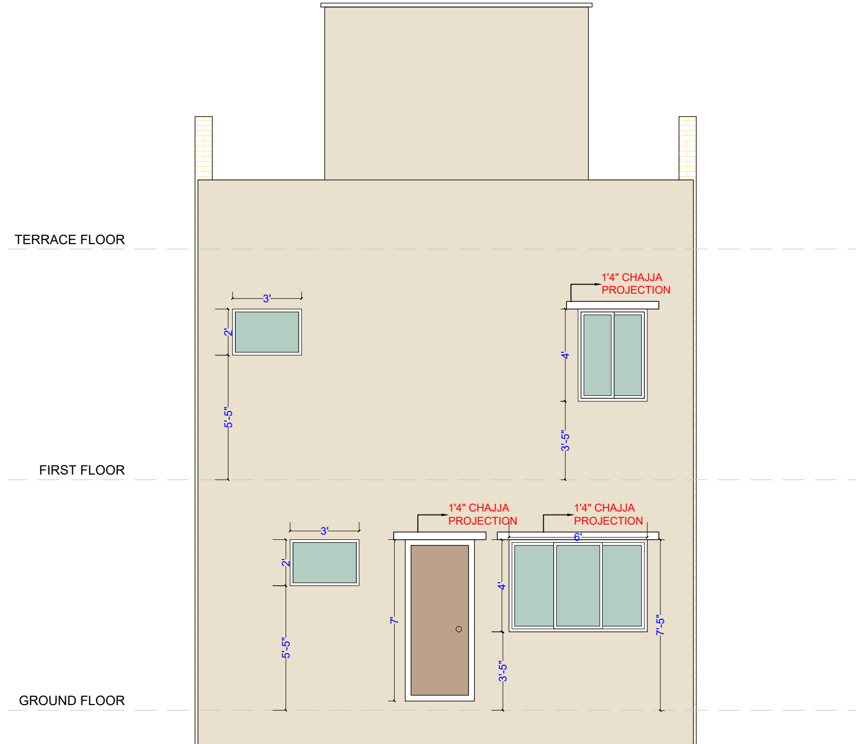
EAST ELEVATION
