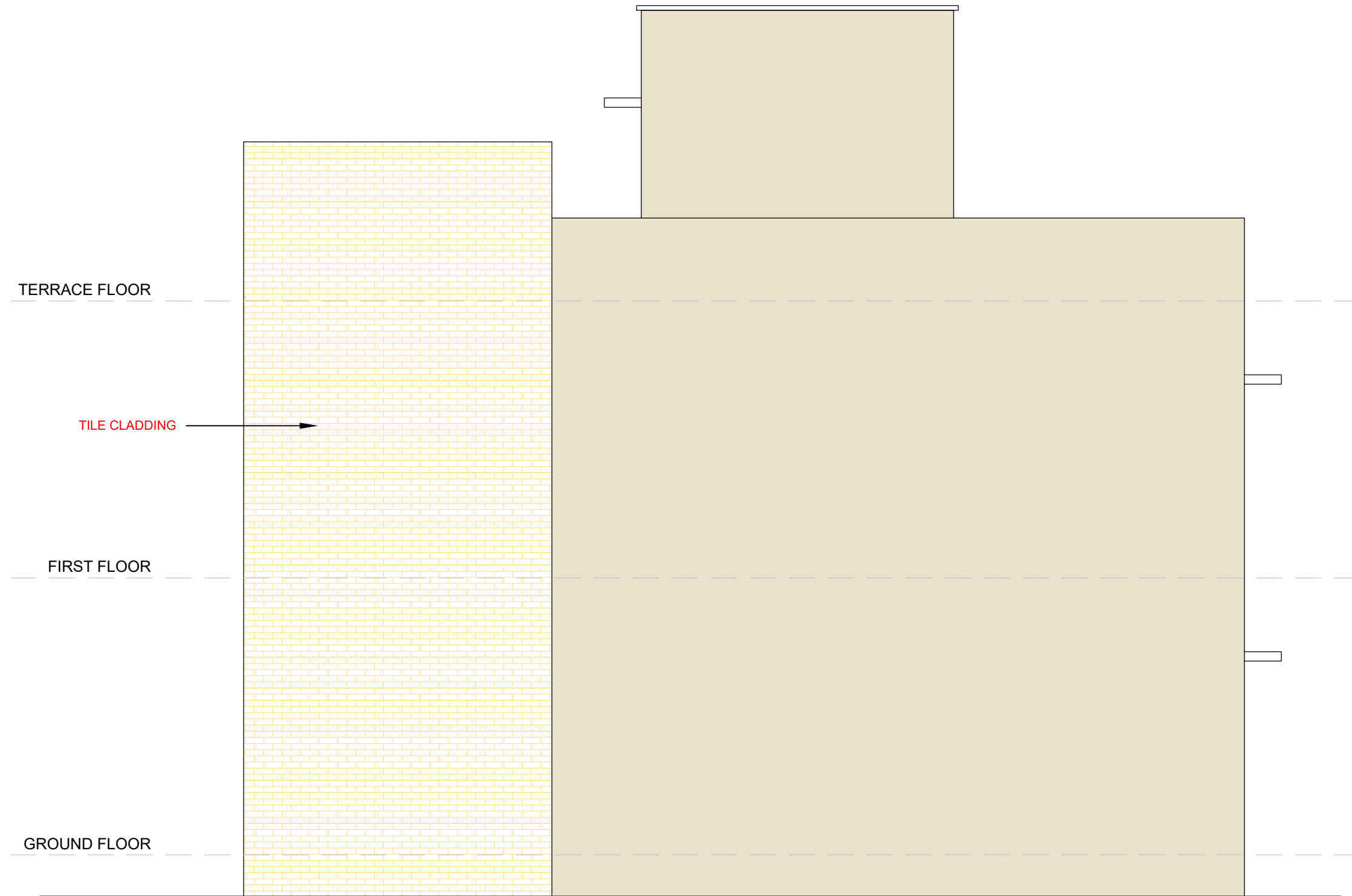
SOUTH ELEVATION
