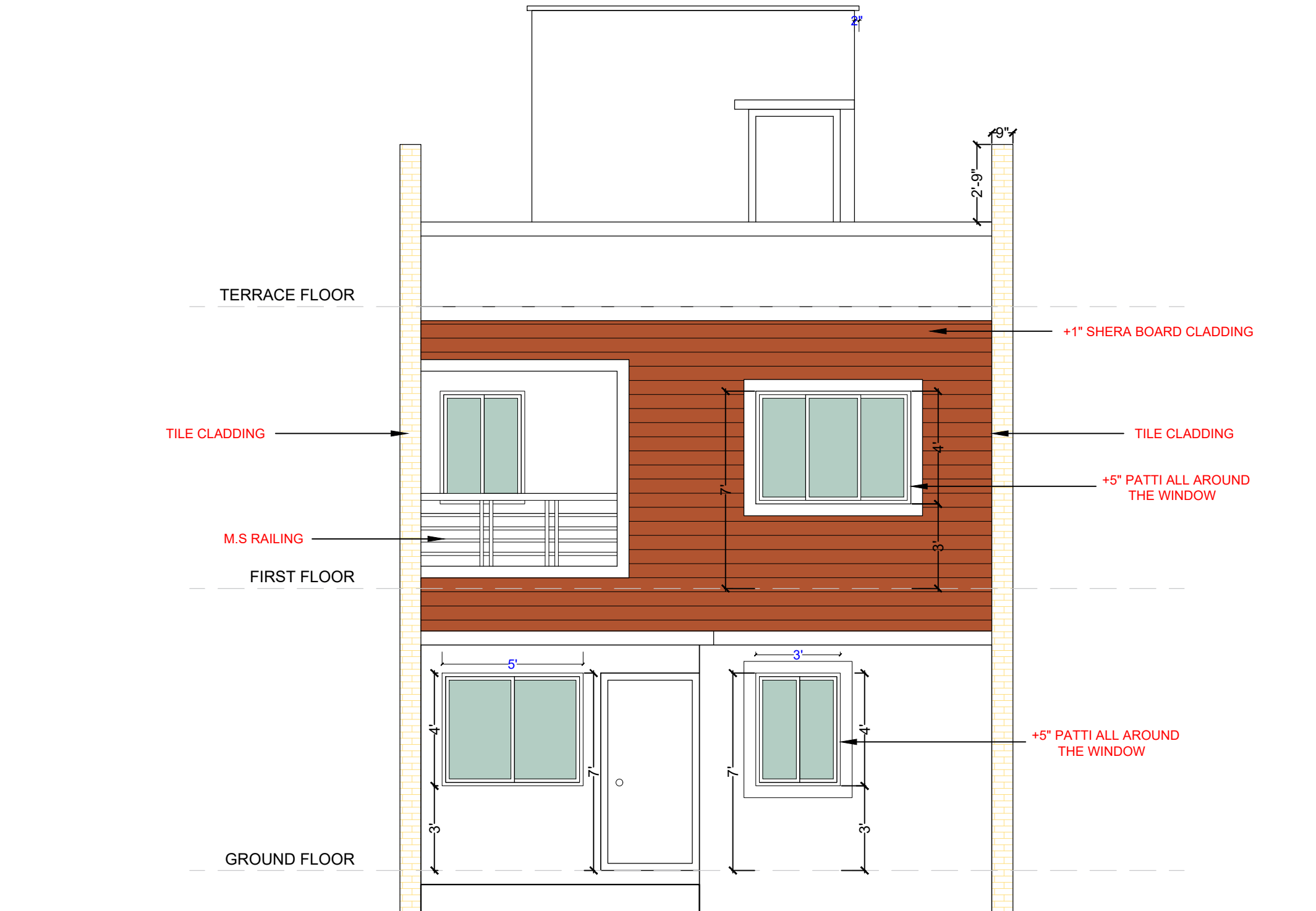
WEST ELEVATION
