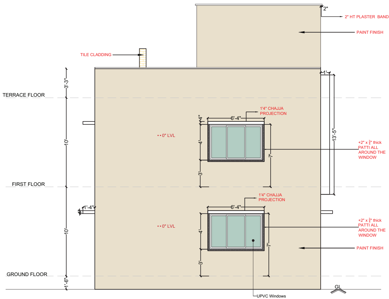
WEST ELEVATION
