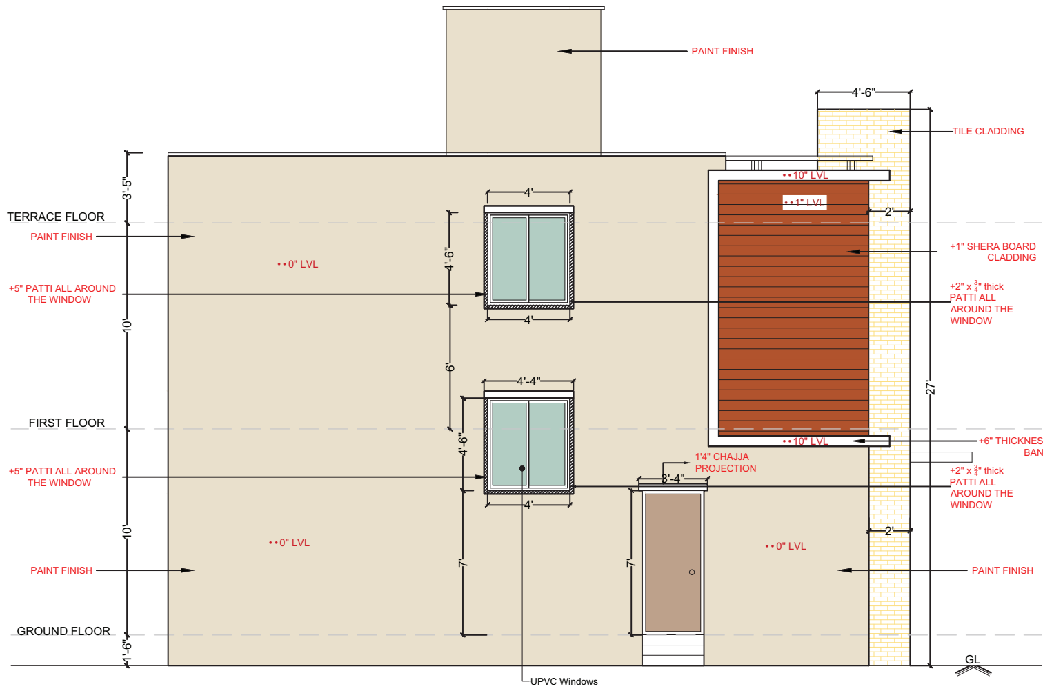
SOUTH ELEVATION
