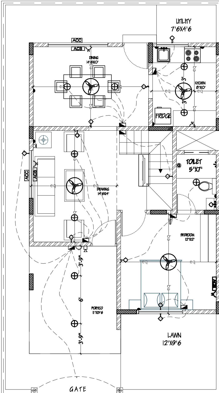
GROUND FLOOR
