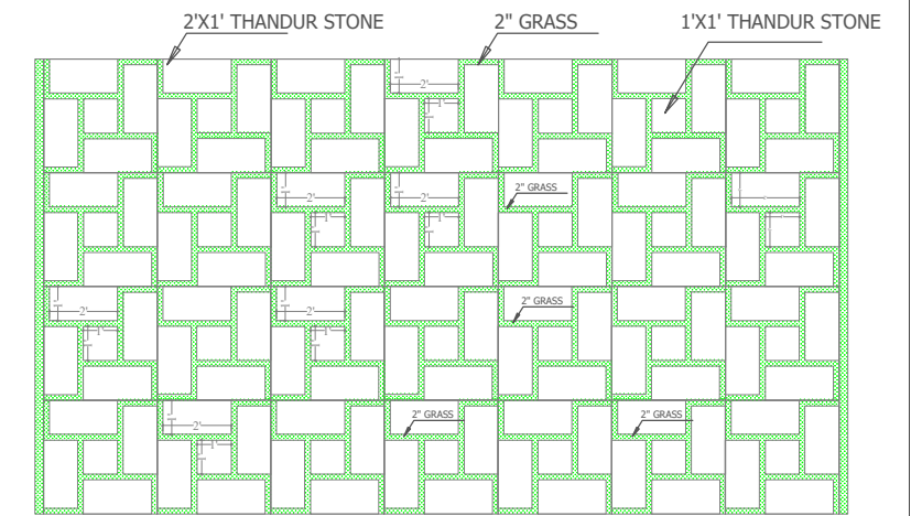
DEATAIL @ A
