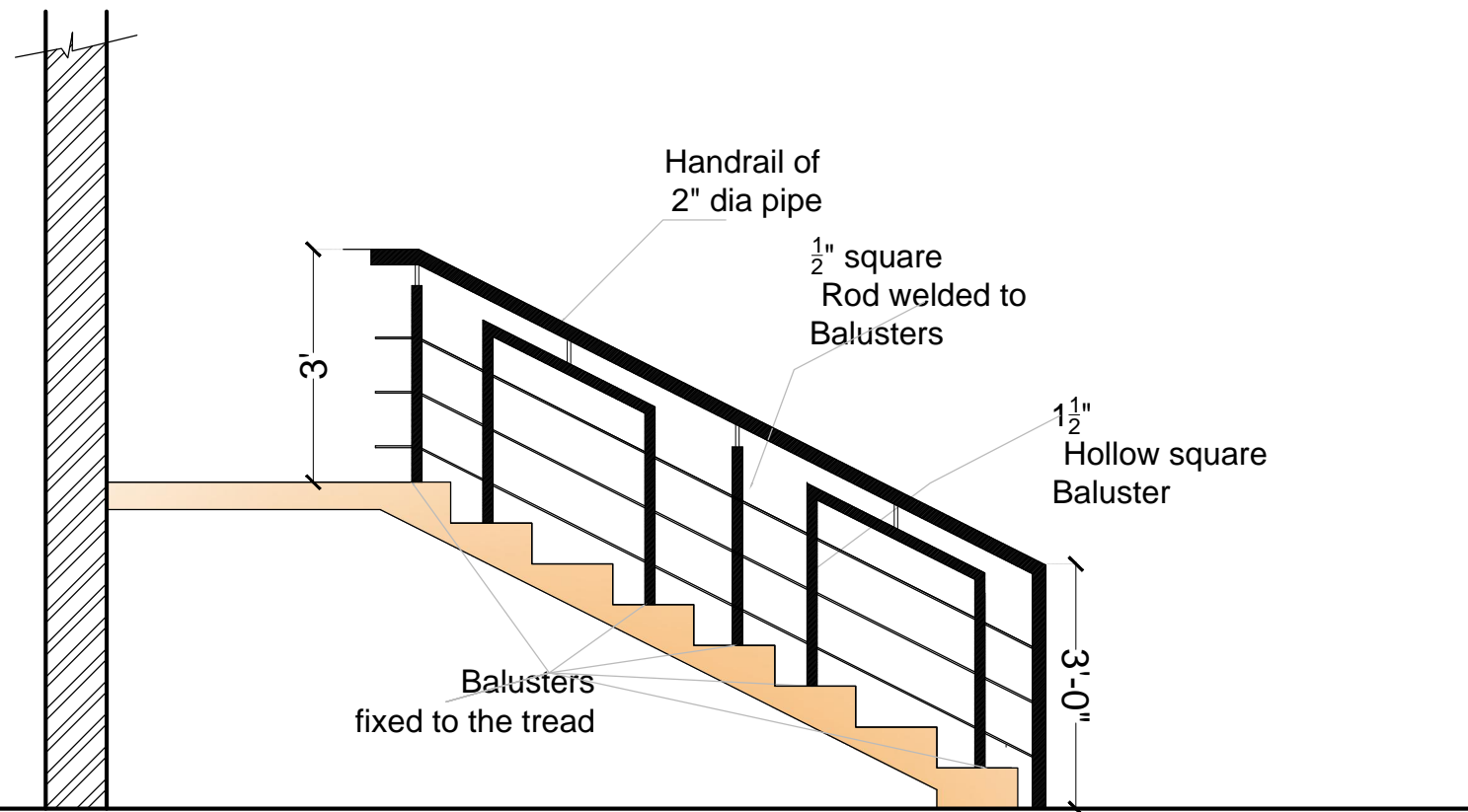
Sectional Elevation-AA (Design option-2)
