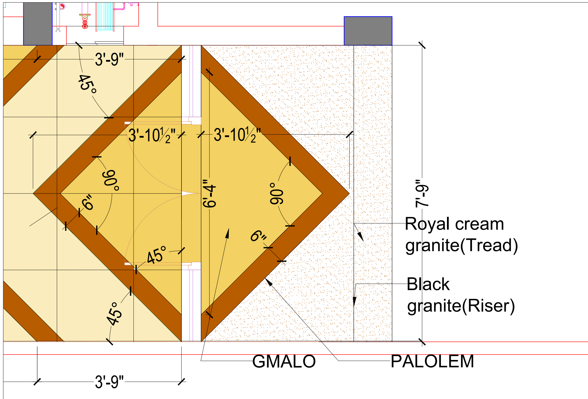
PART PLAN -3
