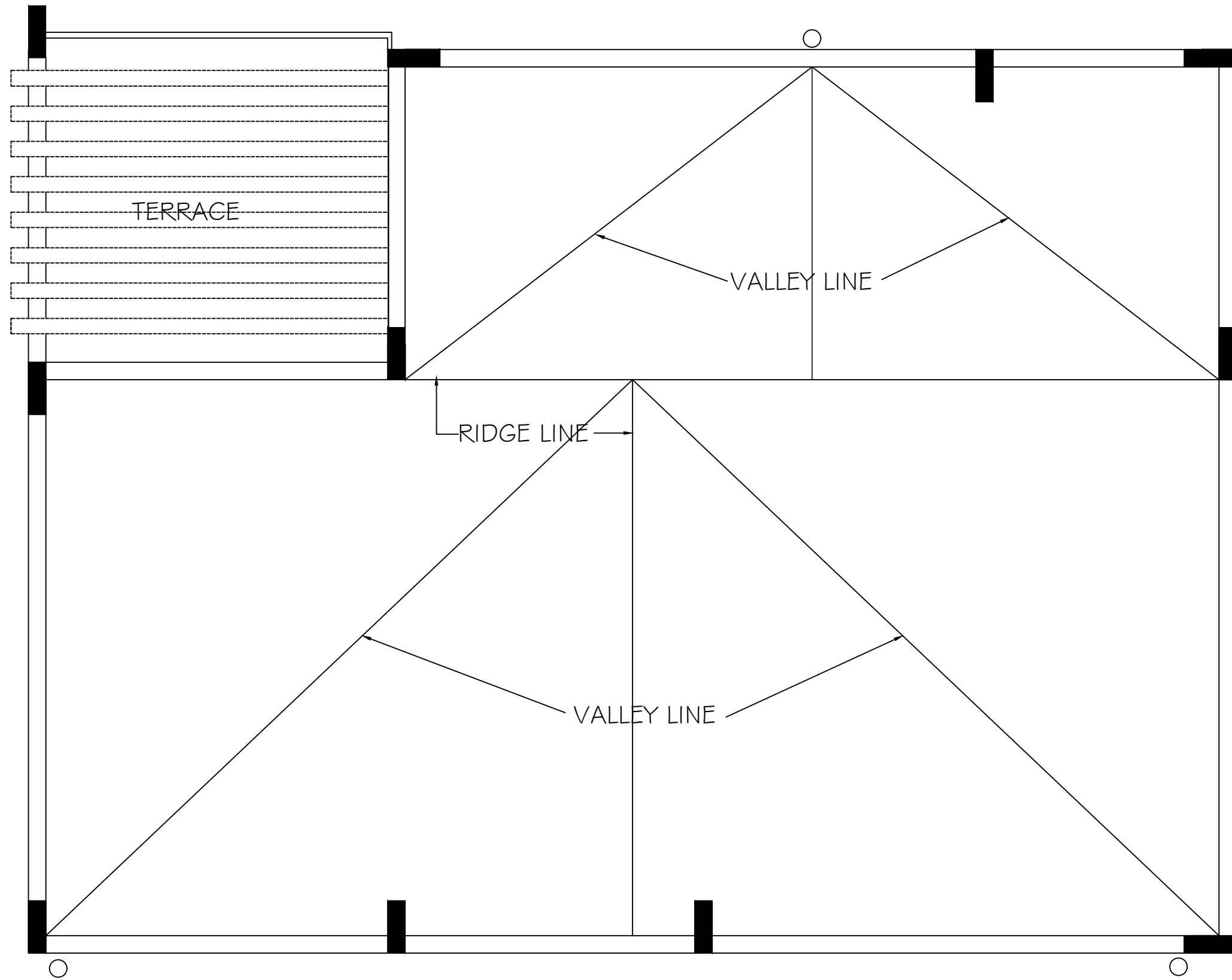
TERRACE PLAN
