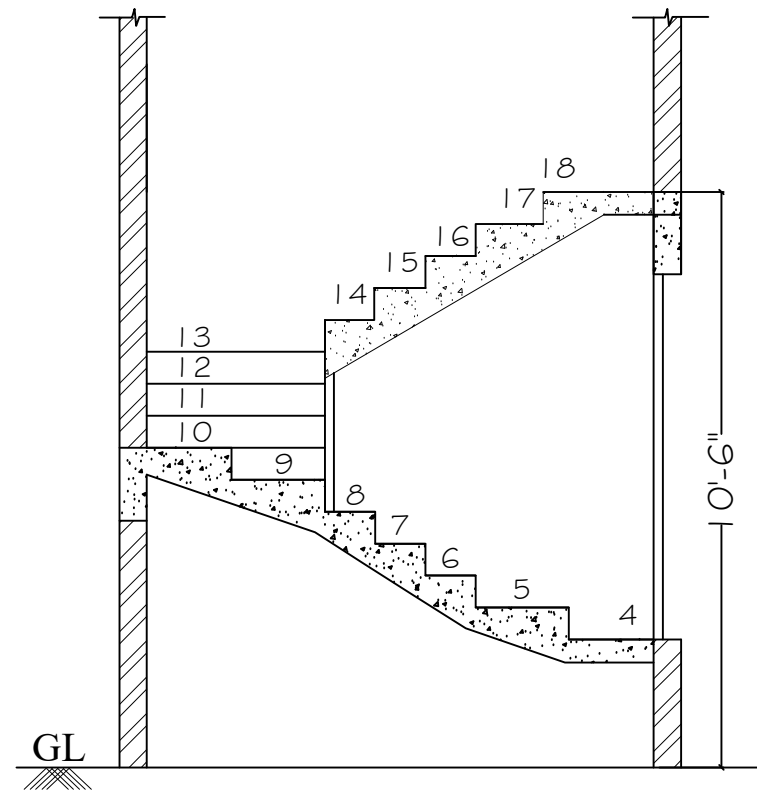
SECTION B-B
