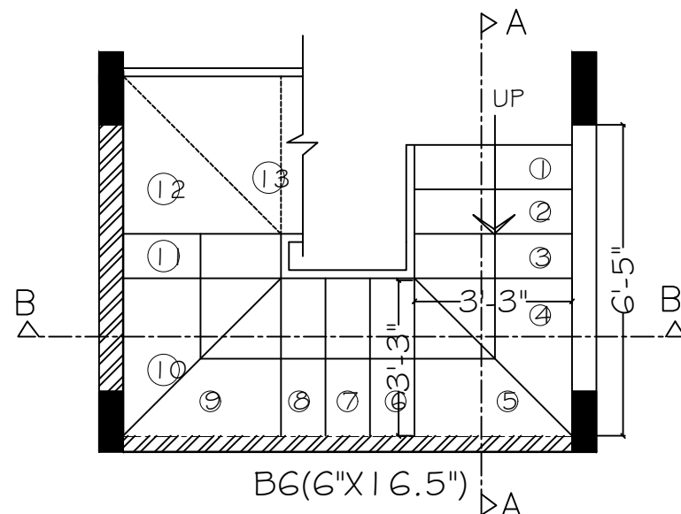
STAIRCASE PLAN
