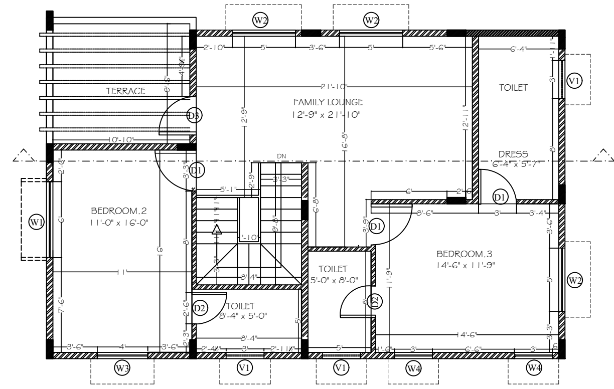
FIRST FLOOR
