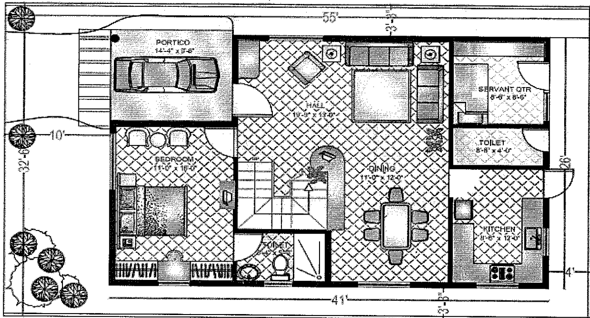
GROUND FLOOR
