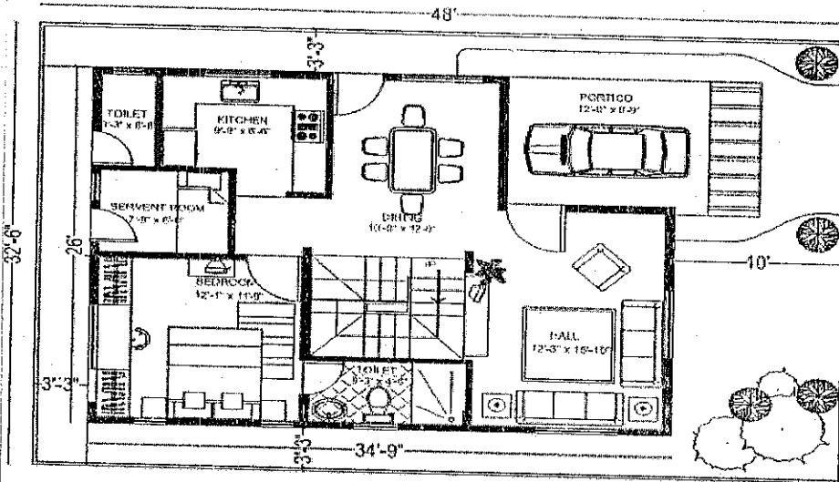
GROUND FLOOR
