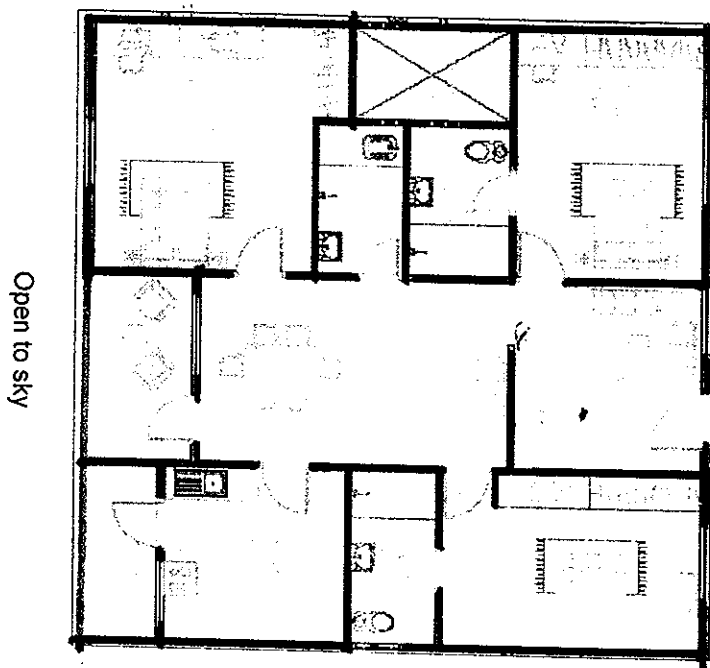
Flat No. 205
