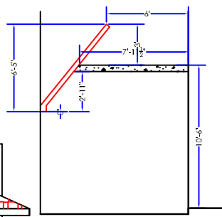
SECTION - X
