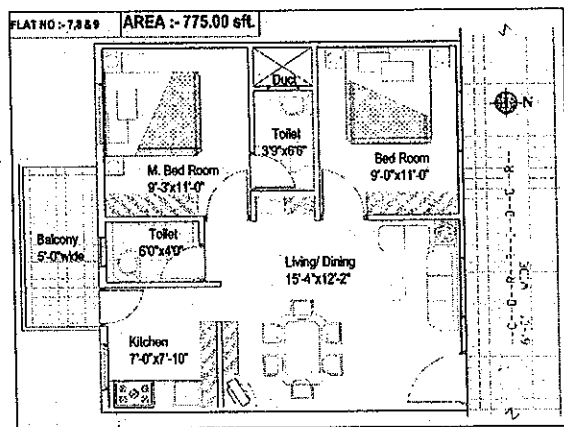
Floor Plan of Apartment
