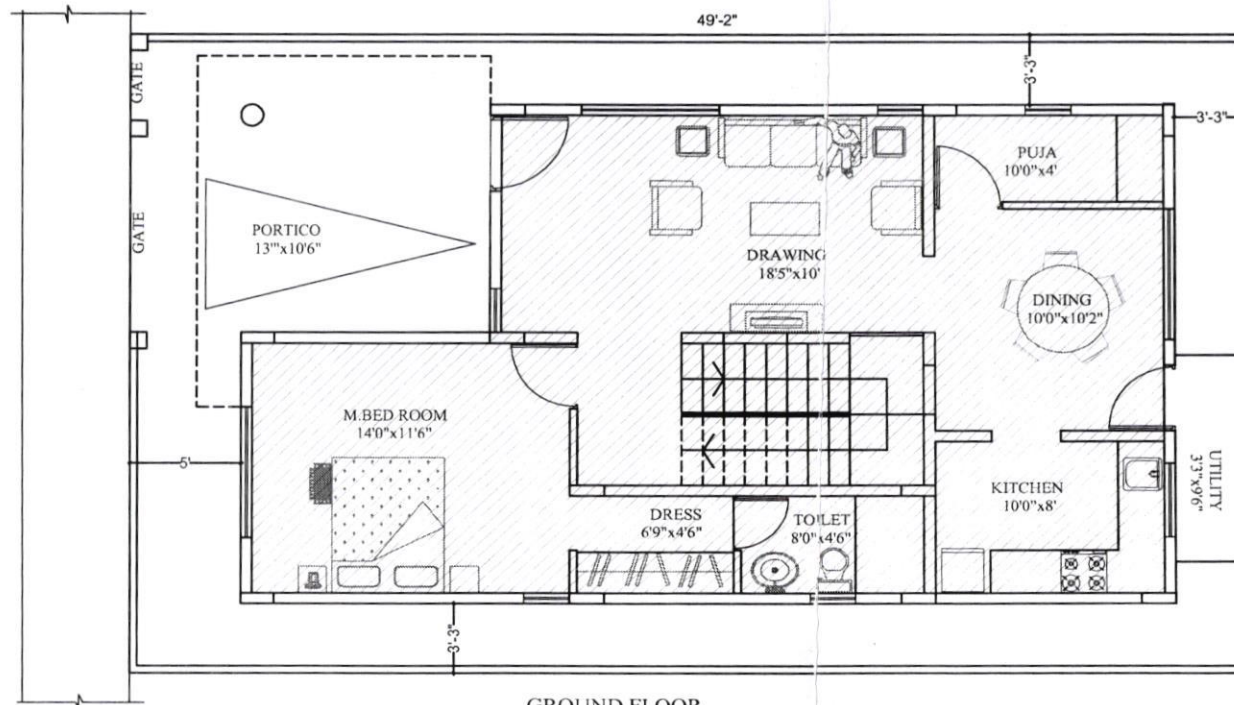
GROUND FLOOR
