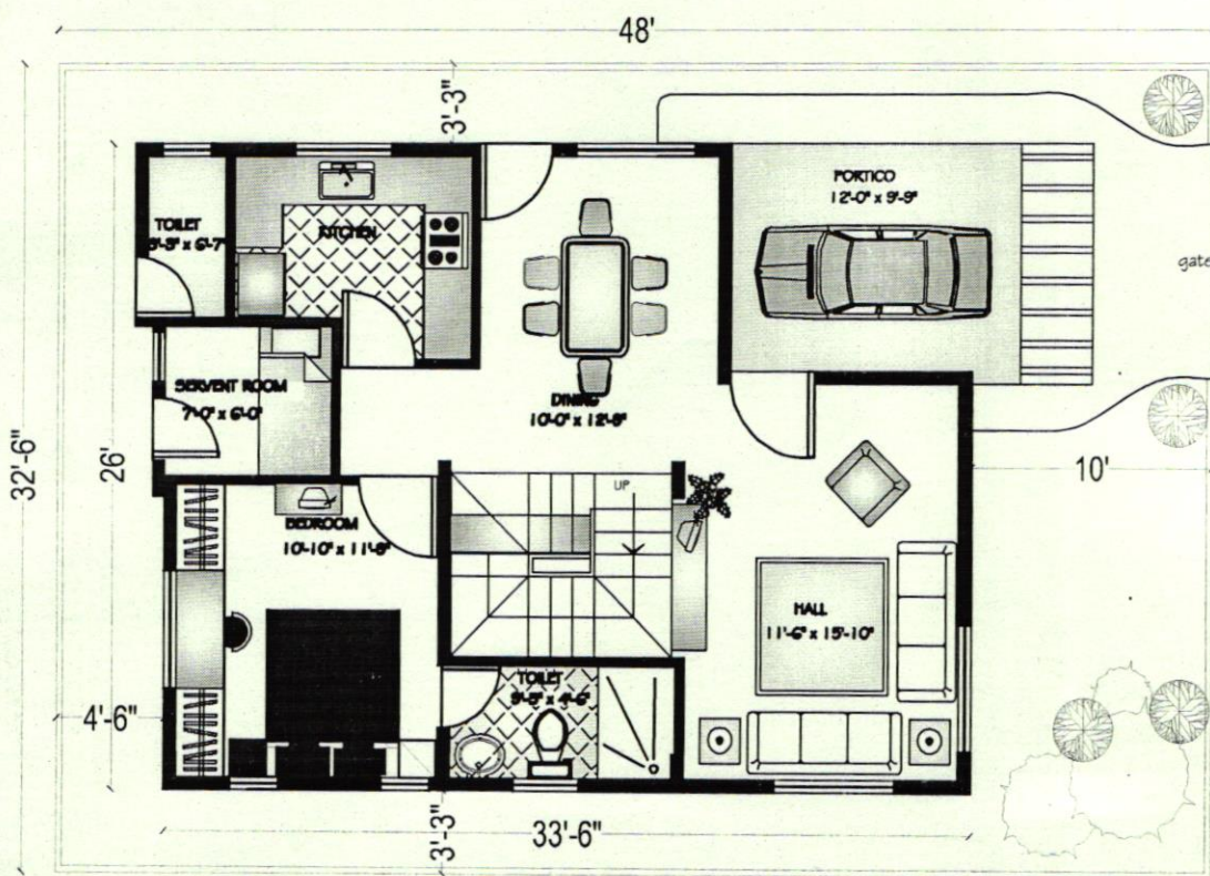
GROUND FLOOR
