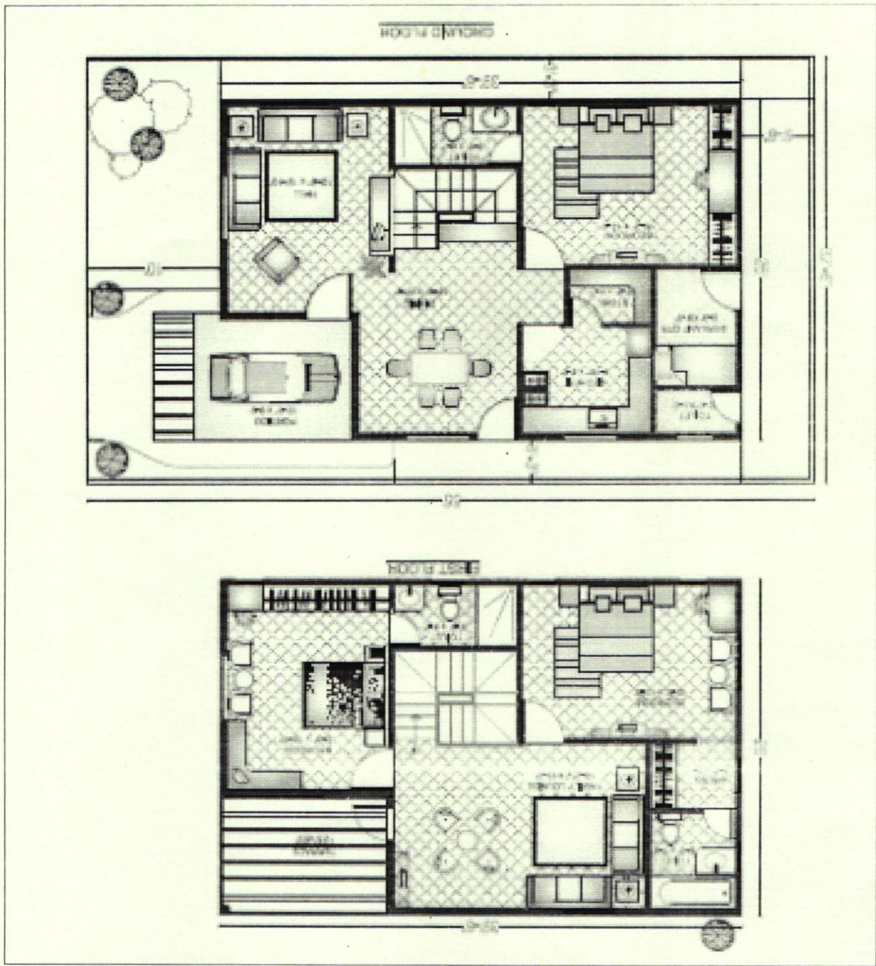
Plan of the Scheduled Villa:
