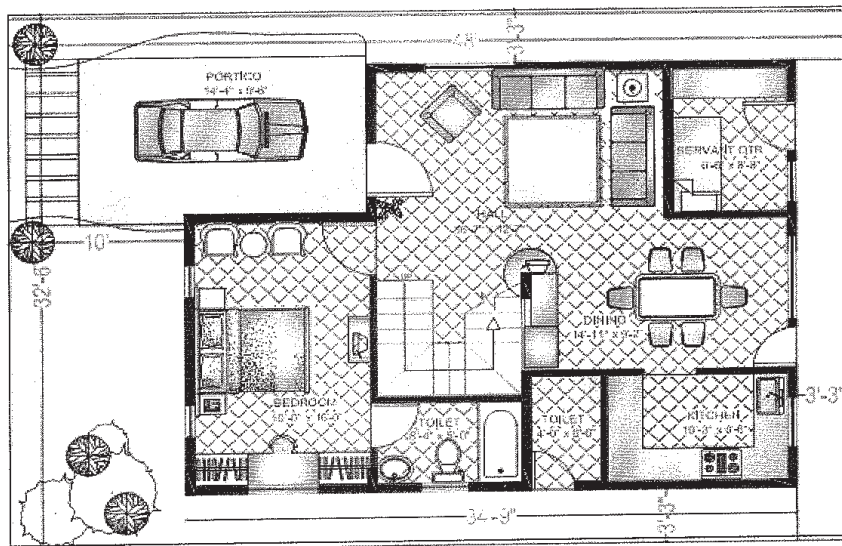
GROUND FLOOR
