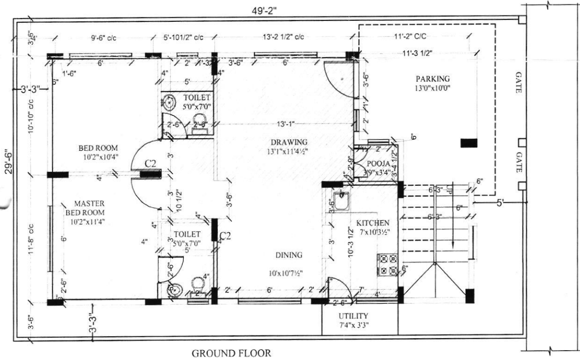
GROUND FLOOR
