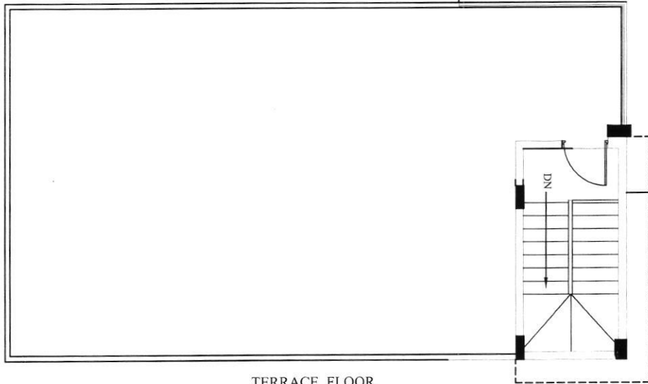
TERRACE FLOOR
