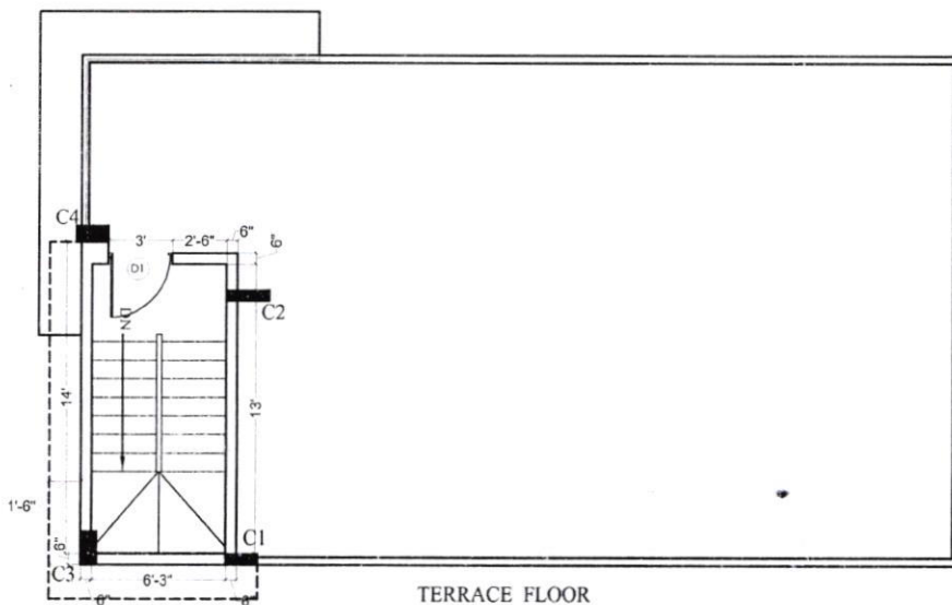
TERRACE FLOOR
