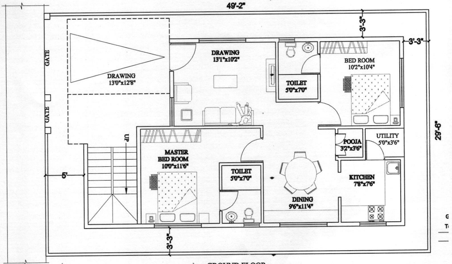
GROUND FLOOR
