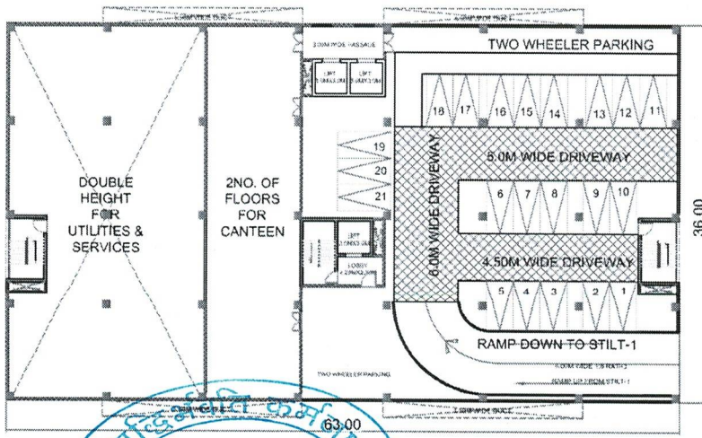
STILT-2 PARKING FLOOR PLAN
