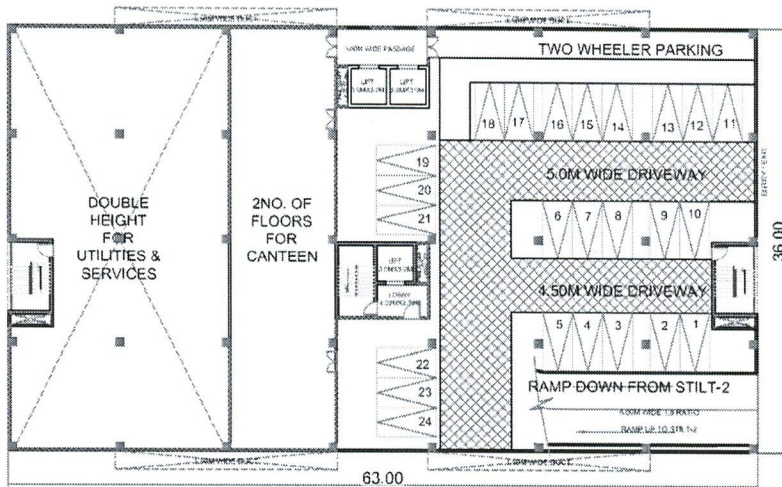
STILT-1 PARKING FLOOR PLAN
