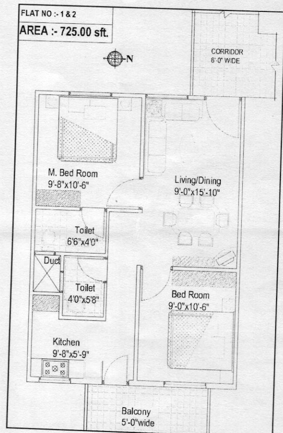
Floor Plan of Apartment
