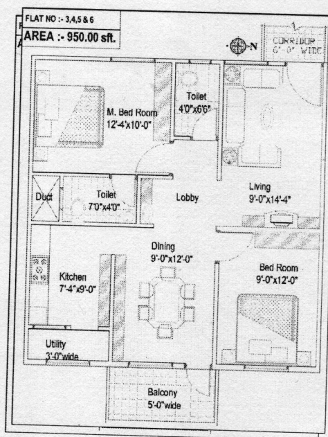
Floor Plan of Apartment
