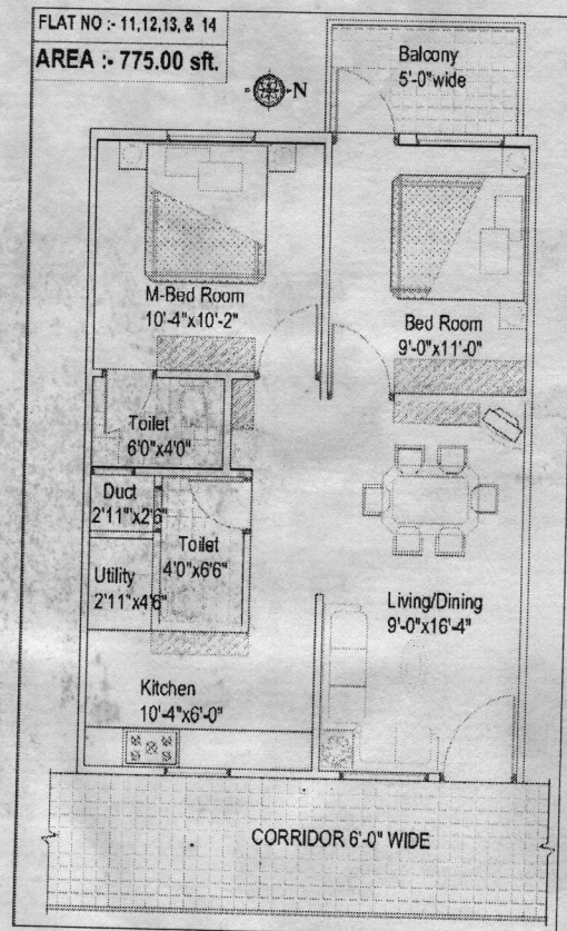
Floor Plan of Apartment
