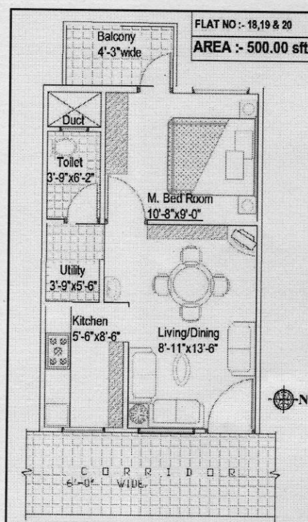
Floor Plan of Apartment
