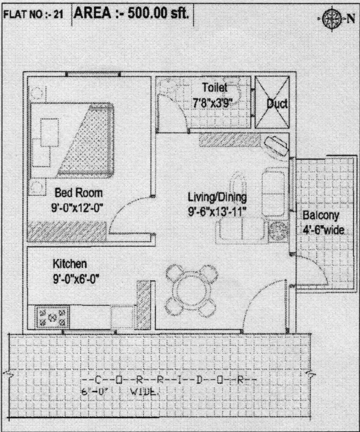
Floor Plan of Apartment
