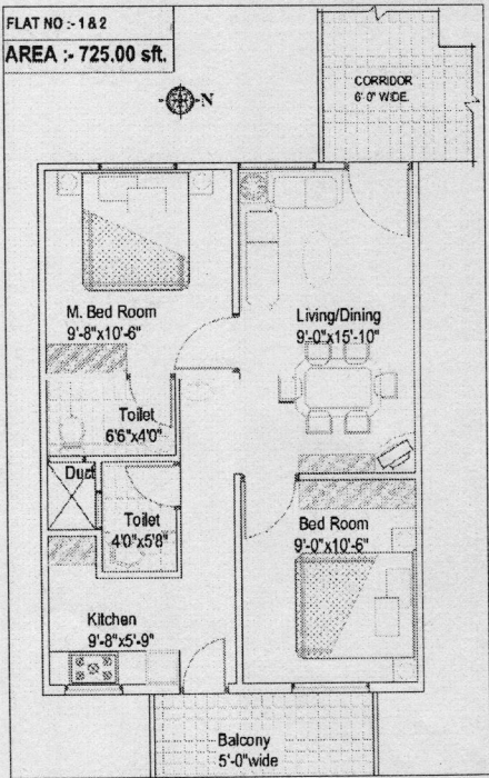
Floor Plan of Apartment
