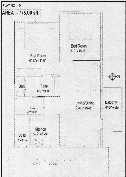
Floor Plan of Apartment
