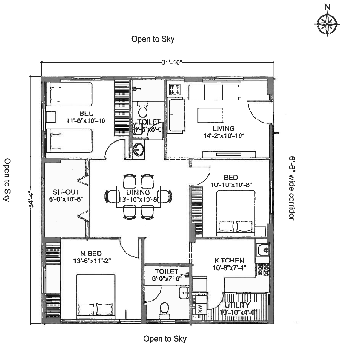
Plan of the Scheduled Flat:
