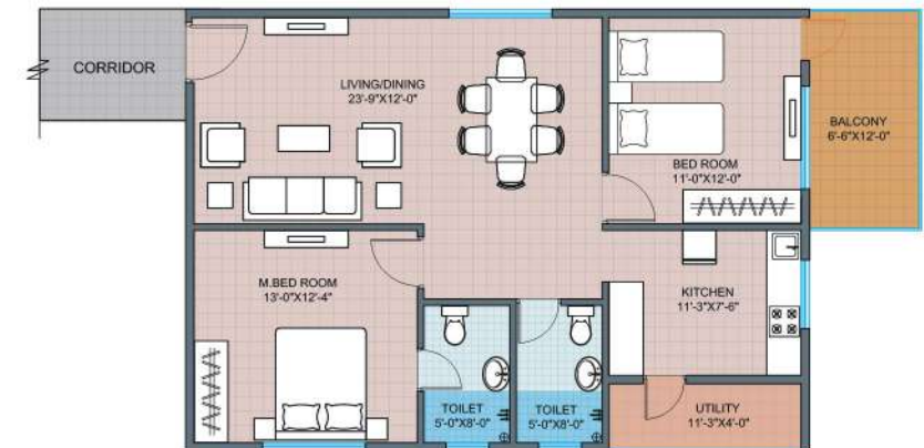
TYPE - VI AREA - 1,220 sq.ft.
