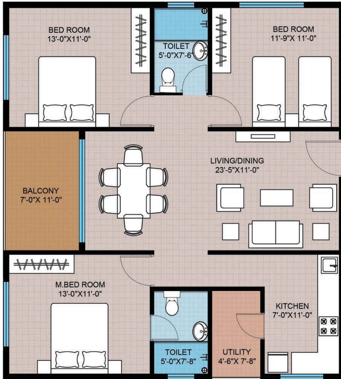
TYPE A1 AREA - 1,360 sft.
