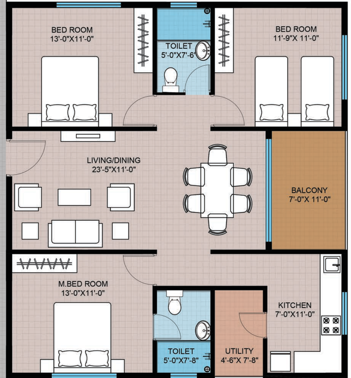
TYPE A2 AREA - 1,360 sft.
