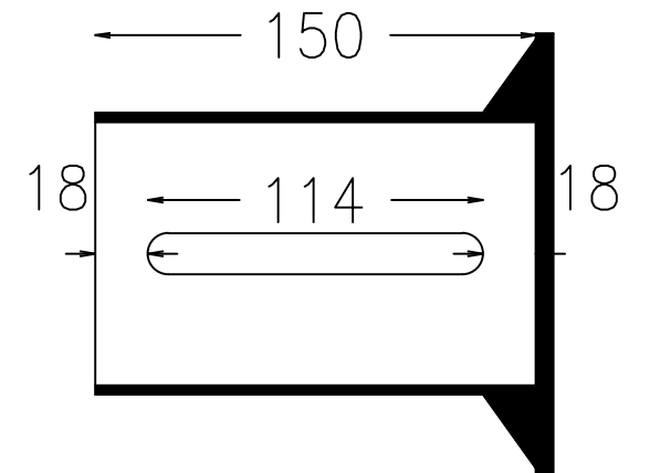
d.Lift Side Bracket
