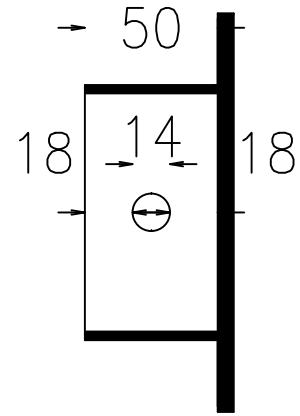
a.Lift Side Bracket
