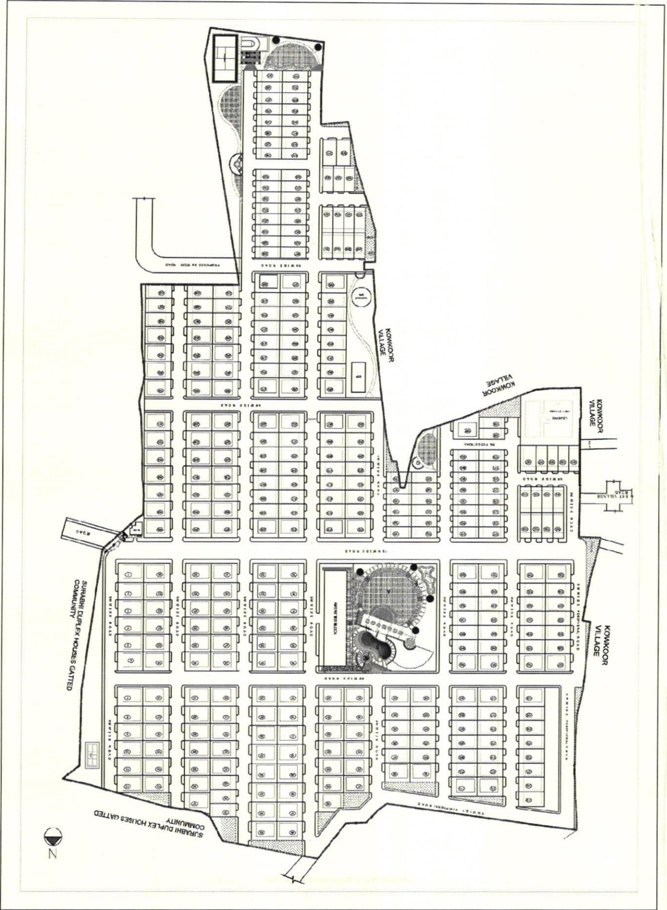
Layout plan of the Housing Project:
