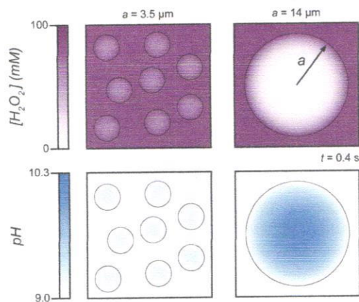
Fig. 6 Computed profiles for \text{H}_2\text{O}_2 concentration (top) and pH (bottom) in and around small (left) and large (right) coacervate droplets at time t = 0.4 s after addition of \text{H}_2\text{O}_2 . The parameters and conditions of the reaction-diffusion model are chosen to match those of the experiments in Fig. 5 (see ESI Section 2.1 and Fig. S3† for details). For droplets smaller than the reaction-diffusion length a^* = 7 \mu\text{m} , \text{H}_2\text{O}_2 diffuses throughout the drop interior before being consumed by the reaction (top, left); the local pH increase within the droplet is limited by diffusive exchange with the surrounding solution (bottom, left). For large drops, peroxide decomposition is localized near the drop interface (top, right), and the local pH rises significantly within the drop interior (bottom, right).
