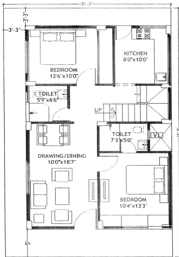
GROUND FLOOR PLAN AREA: 800 SFT
