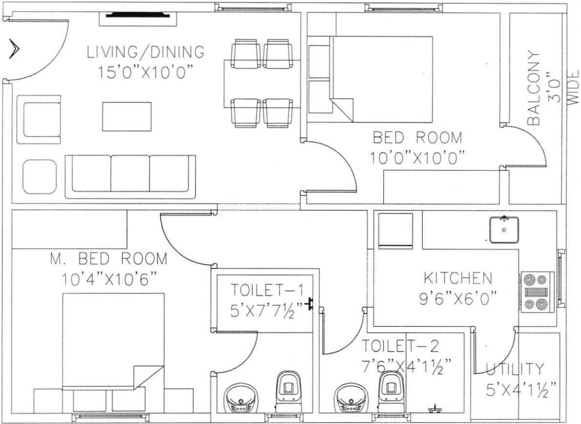
WEST FACING UNIT PLAN
