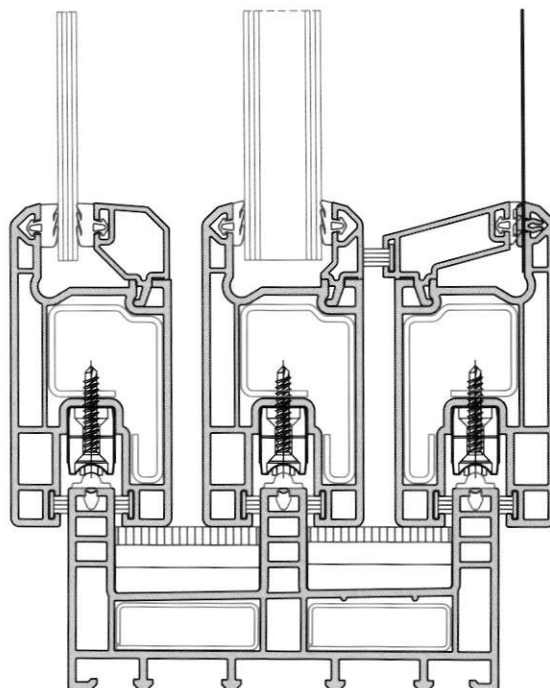
3 TRACK (112 mm)
