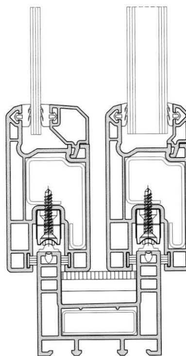
2 TRACK (62 mm)
